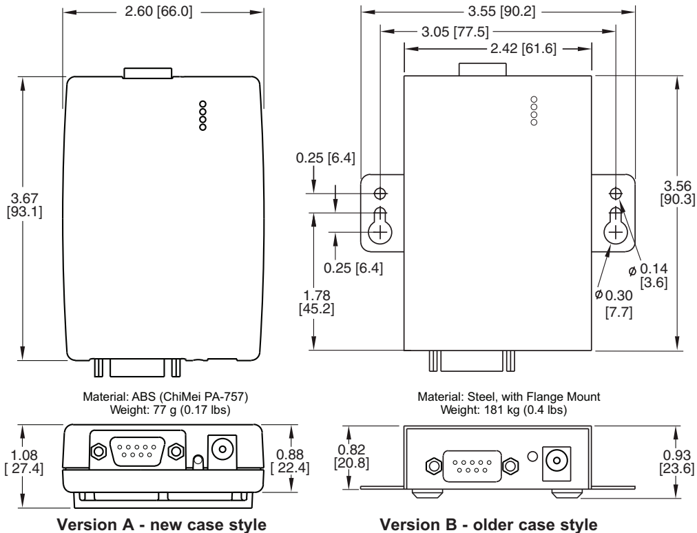
Figure 5.1 Wall Mount iServer Dimensions
